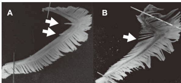
鰓耙
